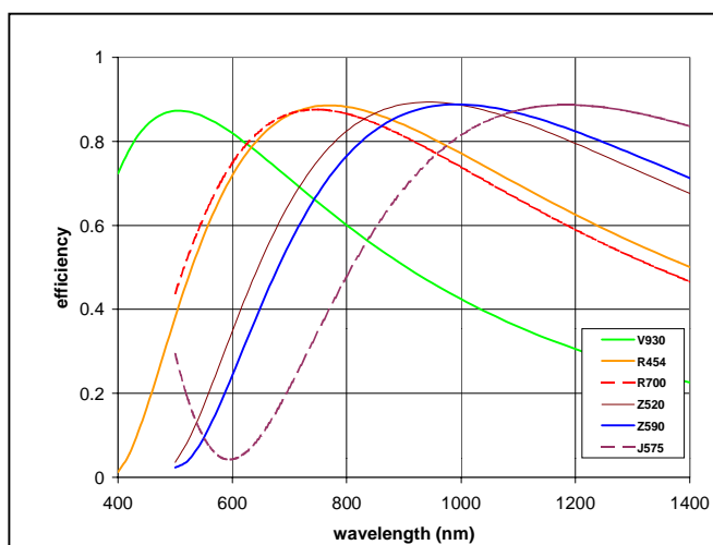
Figure 4. Predicted efficiency curves for a variety of VPH gratings in the visible to near IR wavelength range.
