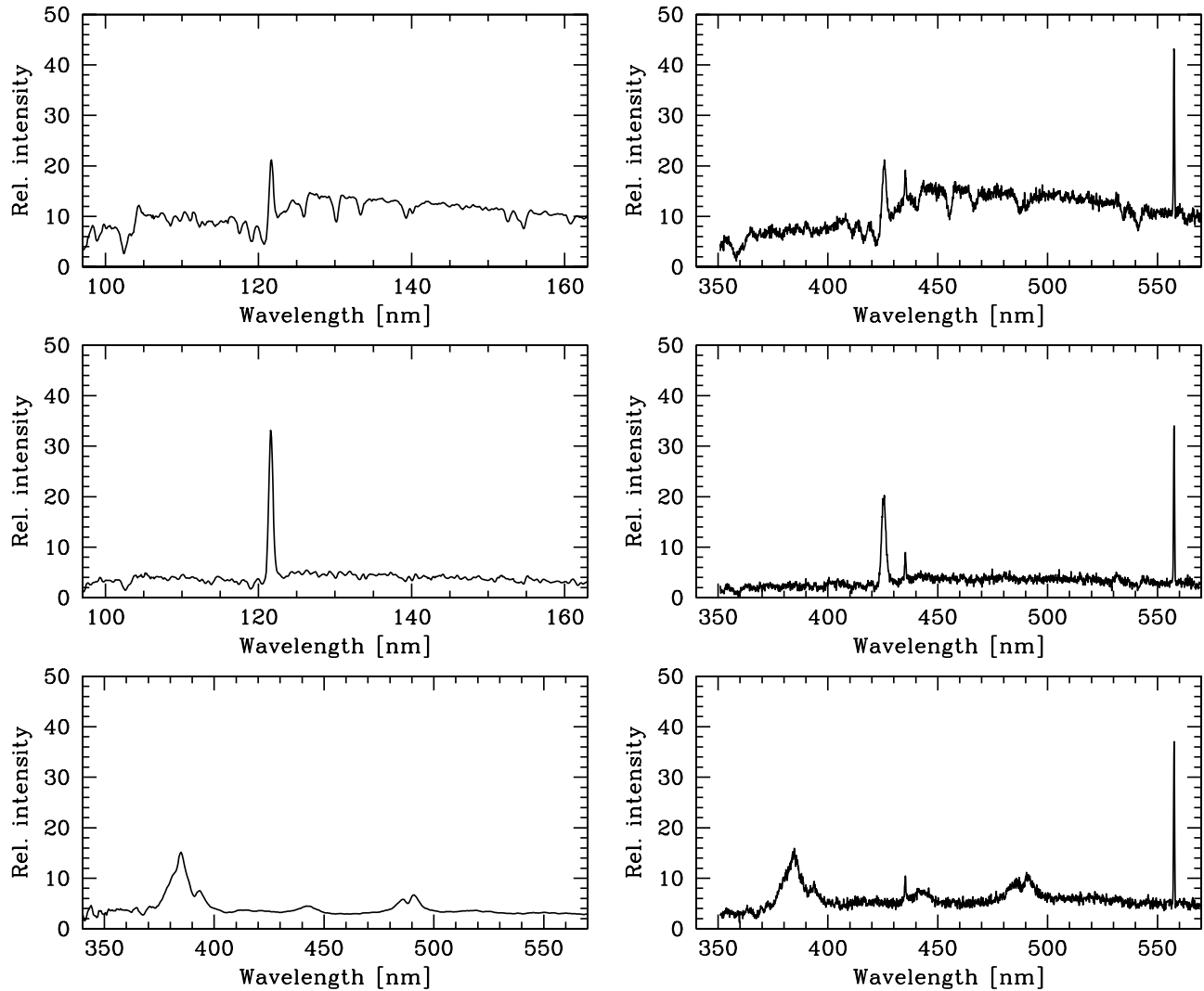
Figure 2. The input (left) and the extracted (right) spectra of Fig. 1. We used an adjusted version of the PMAS/PPAK software package 13, 14 for extraction and wavelength calibration of the simulated spectra. Top: Weak LAE; left is rest frame template, right is simulation for z = 2.5 . Center: Strong LAE; left is rest frame template, right is simulation for z = 2.5 . Bottom: QSO at z = 2.1 . The strong line at 577 nm is a bright night sky emission line and clearly visible in all the spectra of Fig. 1.
