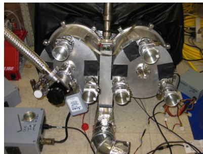
Figure 7. The adjuster back shown installed on a VIRUS camera. The adjuster back is a modified cryostat cover. The top portion has been cut away and refit with two caps which allow KF25 ports to bolt on, as well as vacuum windows to view each hex key. In this photo the windows are covered with black masks for imaging. The caps have been welded to the cryostat cover.
